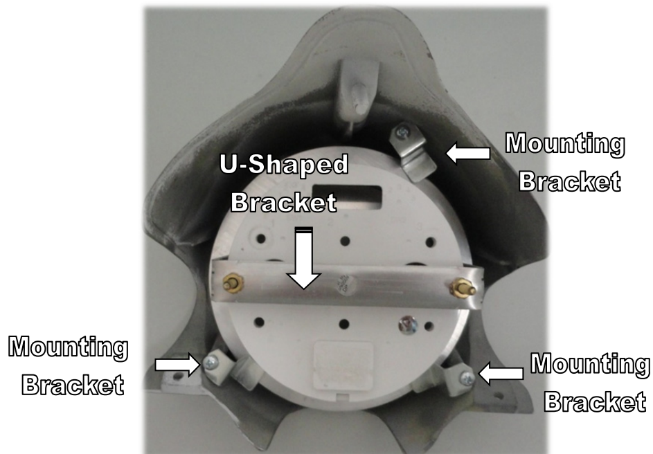
Fig 3: Assembled Center Gauge Pod
