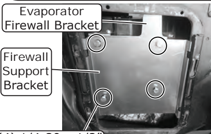
(4) 1/4-20 x 1/2" Hex Bolts
