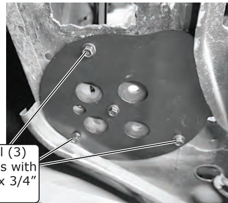
Engine Compartment View Photo 4
